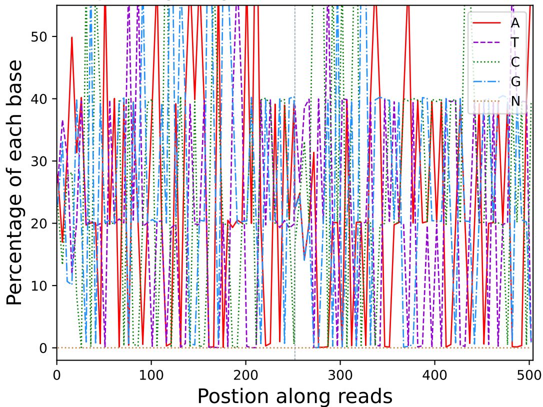
Base percentage along reads (R10115)
